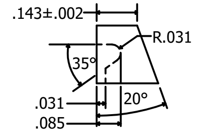
GASKET GROOVE 14WMP-1/2"
